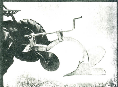
MOLDBOARD PLOW: Single furrow plow, available in both 9" and 10" bottoms. Fully adjustable for depth and leveling. Rolling coulters available to match.
